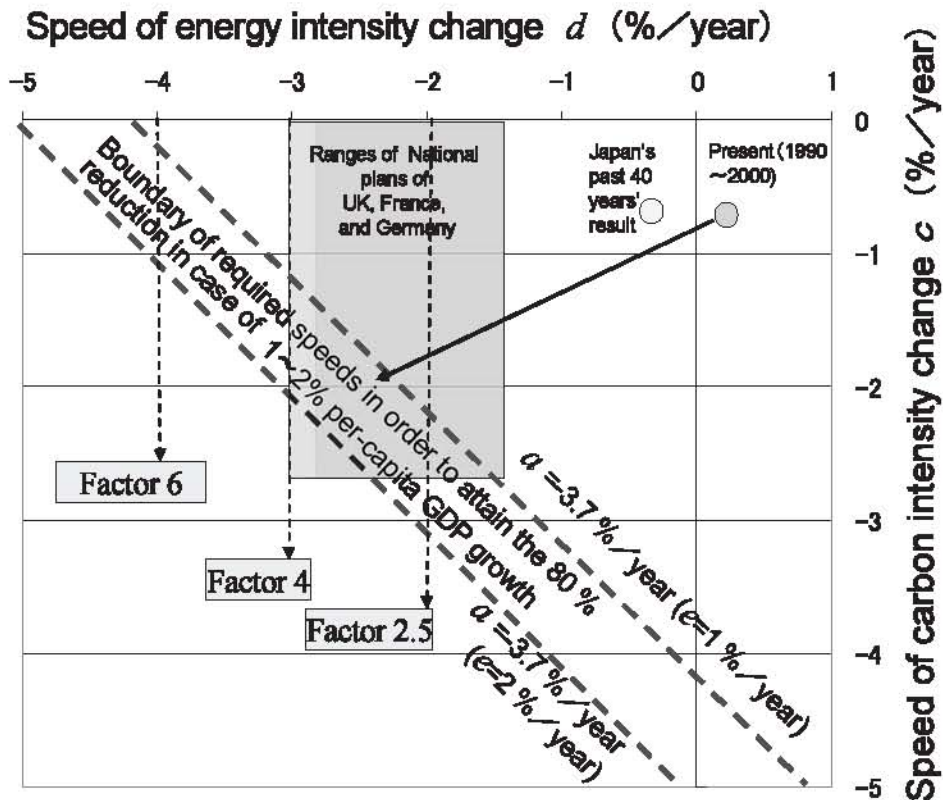
Fig. 6 Speeds required to reduce emissions by 80% by 2050 in Japan
