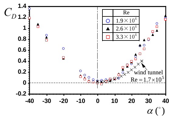
Fig. 8 Profiles of drag coefficient
