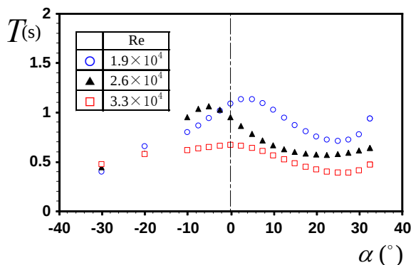
Fig. 16 Relationship between oscillation period and attack angle
