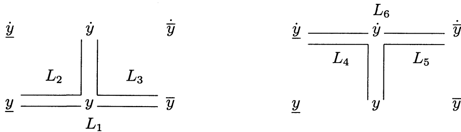
Figure 1: Lax equations
