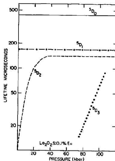
Fig. 16. Lifetimes vs. pressure— {}^3D levels of \text{Eu}^{+3} in \text{La}_2\text{O}_2\text{S} .
