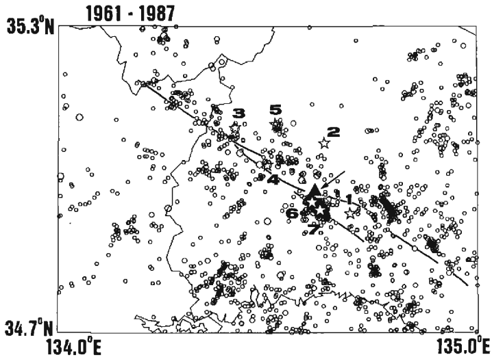
Fig. 3a. Distribution of microearthquakes of M \geq 1.6 and H \leq 40 km obtained by the Tottori Microearthquake Observatory 16) , from 1961 to 1987. Asterisks with numerals denote the epicenters of M \geq 5 determined by J. M. A., from 1926 to 1987. The solid lines and the solid triangle with an arrow show the Yamasaki fault and the Yamasaki Fault Observation Station, respectively.
