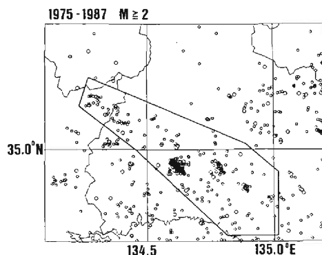
Fig. 13a. Epicentral distribution of earthquakes of M \geq 2.0 and H \leq 40 km obtained by the Tottori Microearthquake Observatory network. The seismic activities of the surrounding area is discussed, in which the Yamasaki fault is wholly included.
