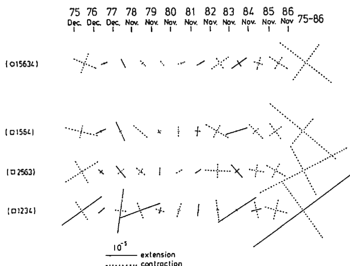
Fig. 14. Strain variations obtained by geodetic measurements. (After Omura et al.; 1988) 38)
