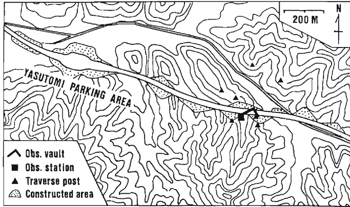
Fig. 2. Topography around the Yamasaki Fault Observation Station (■). The Chugoku Expressway lies east-west near the station and the Yasutomi Observation Vault (L-shaped) has been situated just under the expressway. Solid triangles denote the traverse posts of the Yasutomi–Usuzuku Baseline Network for geodetic measurements.
