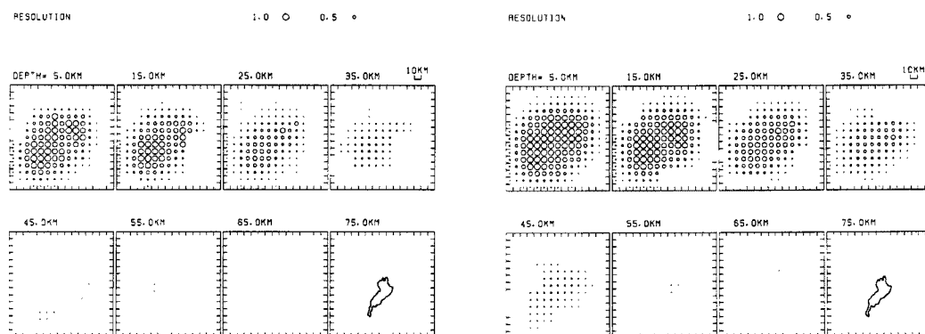
Fig. 4. Resolution of scattering strength inversion in the case of using (a) six routine stations only and (b) those added ten temporary stations. Diagonal element of resolution matrix is plotted for each block, with rough illustration of the location of Lake Biwa at the lowermost layer.
