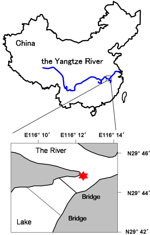
Fig. 1 Map of survey area: the convergent area of Poyang Lake and the Yangtze River. The star shows the observation site.
