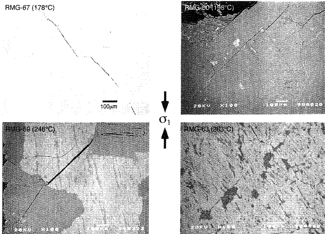
Fig. 4 Typical examples of SEM micrographs (backscattered electron images) of the high-pressure type cracks at a confining pressure of 1500 MPa. The direction of the compressive stress is vertical.
