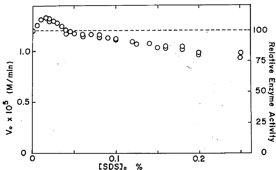
Fig. 4.10. Effect of SDS on the hydrolysis of p -nitrophenyl acetate by subtilisin BPN'. [\text{subtilisin BPN}']_0 = 4.49 \mu\text{M} , and [\textit{p}\text{-nitrophenyl acetate}]_0 = 0.394 \text{ mM} in 25 mM phosphate buffer, pH 7.0, ionic strength 0.1 M (NaCl) containing 5.0% (v/v) isopropanol at 25.0°C.
