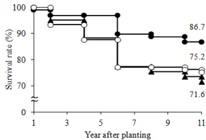
Fig. 5-3. Survival curve of planted Shorea johorensis for 11 years after planting in each three monitoring plots.
