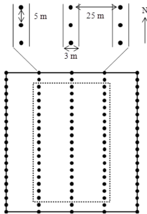
Fig. 5-1. Planting scheme in the 1-ha monitoring plot. Dots represent the planted seedlings. Planted trees within the broken line were used in the evaluation of the crown illumination level using the three-dimensional model.
