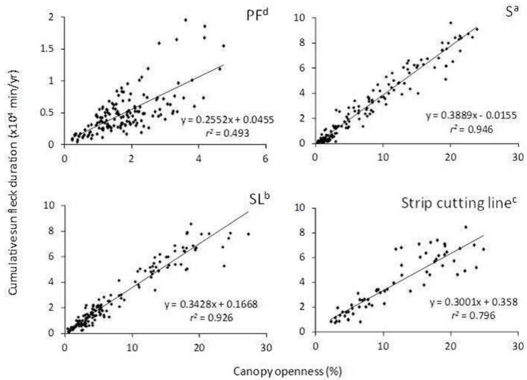
Fig. 3-6. Scatter diagram of the correlation between the calculated canopy openness and cumulative sun-fleck duration for 1 year at each photography point in the primary forest (PF), selective logging (S), and selective logging and line planting (SL) sites and strip cutting lines. Different letters attached to site name indicates statistical difference using Bonferroni's test.
