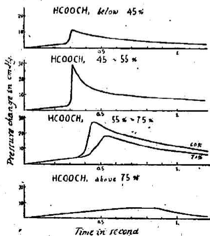
Fig. 3. Pressure-Time Curve.
