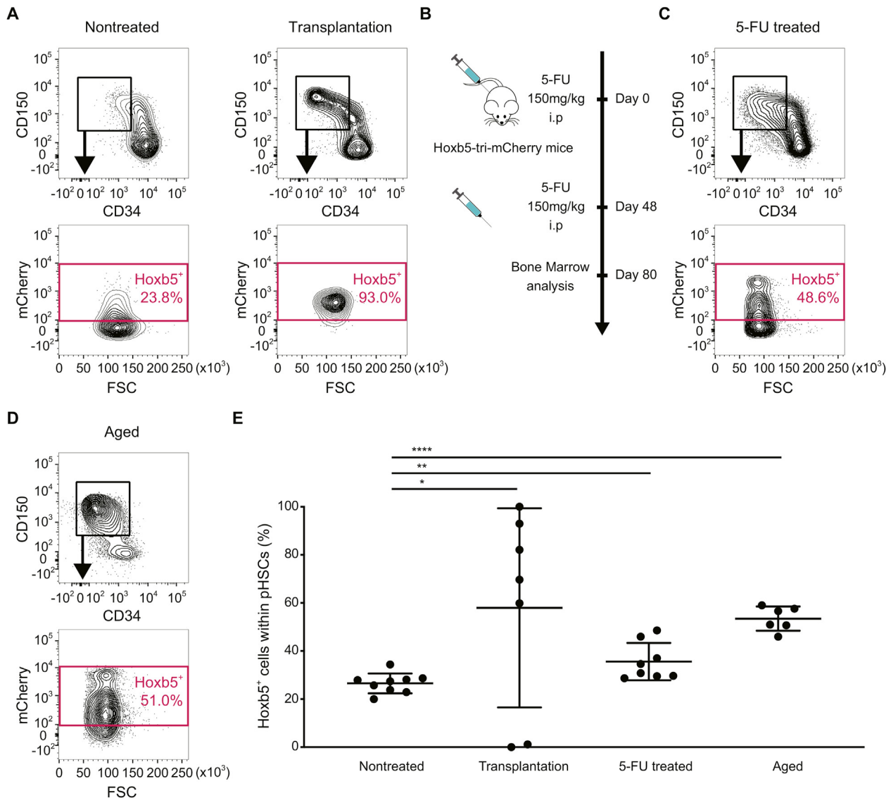
Fig. 2. Selection of Hoxb5 + pHSC in settings of varying stress. (A) Flow cytometry plots of bone marrow from 24-week-old mice transplanted with 10 Hoxb5 + pHSCs (CD45.2 + ) and 2 \times 10^5 supporting cells (CD45.1 + /45.2 + ) 16 weeks before ( n = 7 ) compared with that from 12-week-old Hoxb5-reporter mice. (B) Experimental schematic for 5-FU treatment. After intraperitoneal 5-FU injection (3mg/time; 150 mg/kg) at Day 0 and Day 48, analyze bone marrow at Day 80. (C) Flow cytometry analysis for frequency of Hoxb5 + (mCherry + ) pHSCs in the bone marrow from 20-week-old mice 12 weeks after 5-FU treatment ( n = 8 ). (D) Flow cytometry analysis for frequency of Hoxb5 + (mCherry + ) pHSCs bone marrow from 2-year-old mice. ( n = 6 ). (E) Summarized data about frequencies of Hoxb5 positive cells within pHSCs ( n = 9 for untreated, n = 7 for transplantation, n = 8 for 5-FU, n = 6 for aged).
