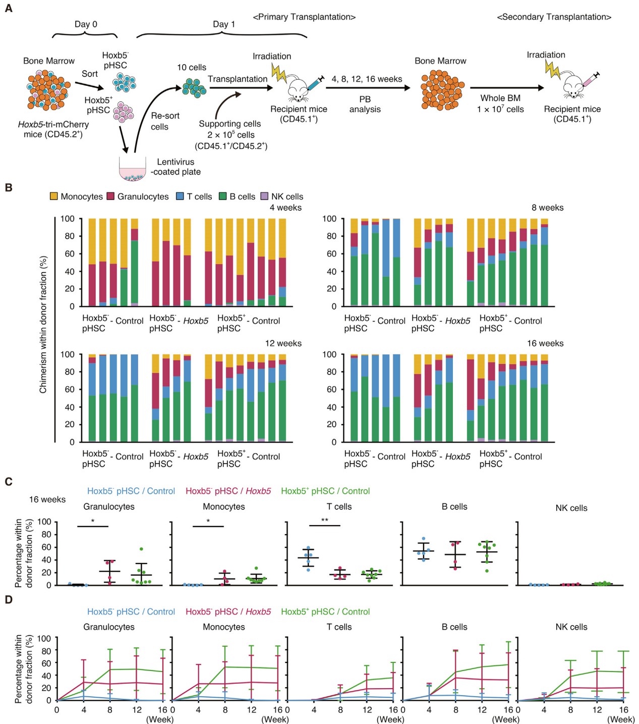
Fig. 4. Exogenous Hoxb5 expression reinforces self-renewal capacity. (A) Experimental schematic for lentiviral transduction of Hoxb5 + pHSCs. Transduced cells were used for transplantation assays. Ten donor cells ( Hoxb5 + or Hoxb5 + pHSCs) were transplanted along with 2 \times 10^5 whole bone marrow cells from CD45.1/CD45.2 mice into lethally irradiated CD45.1 recipient mice. Peripheral blood was analyzed every four weeks. For secondary transplants, 1 \times 10^7 whole bone marrow cells were transferred from the primary recipient mice. (B) Peripheral blood chimerism at 4, 8, 12, and 16 weeks in recipients receiving 10 transduced Hoxb5 + or Hoxb5 + pHSCs along with 2 \times 10^5 whole bone marrow cells from CD45.1/CD45.2 mice. ( n = 5 for Hoxb5 + pHSCs transduced with ZsGreen control; n = 4 for Hoxb5 + pHSCs transduced with Hoxb5 -ZsGreen; and n = 8 for Hoxb5 + pHSCs transduced with ZsGreen control). Each bar represents an individual mouse. (C) Sixteen-week peripheral blood chimerism in each individual lineage (granulocytes, monocytes, T cells, B cells, and NK cells) within total donor cells ( n = 5 for Hoxb5 + pHSCs transduced with ZsGreen control; n = 4 for Hoxb5 + pHSCs transduced with Hoxb5 -ZsGreen; and n = 8 for Hoxb5 + pHSCs transduced with ZsGreen control). Scatter plots summarize each group. (D) Average donor lineage contribution kinetics in 10 cell primary transplants at 4, 8, 12, and 16 weeks ( n = 5 for Hoxb5 + pHSCs transduced with ZsGreen control; n = 4 for Hoxb5 + pHSCs transduced with Hoxb5 -ZsGreen; and n = 8 for Hoxb5 + pHSCs transduced with ZsGreen control).
