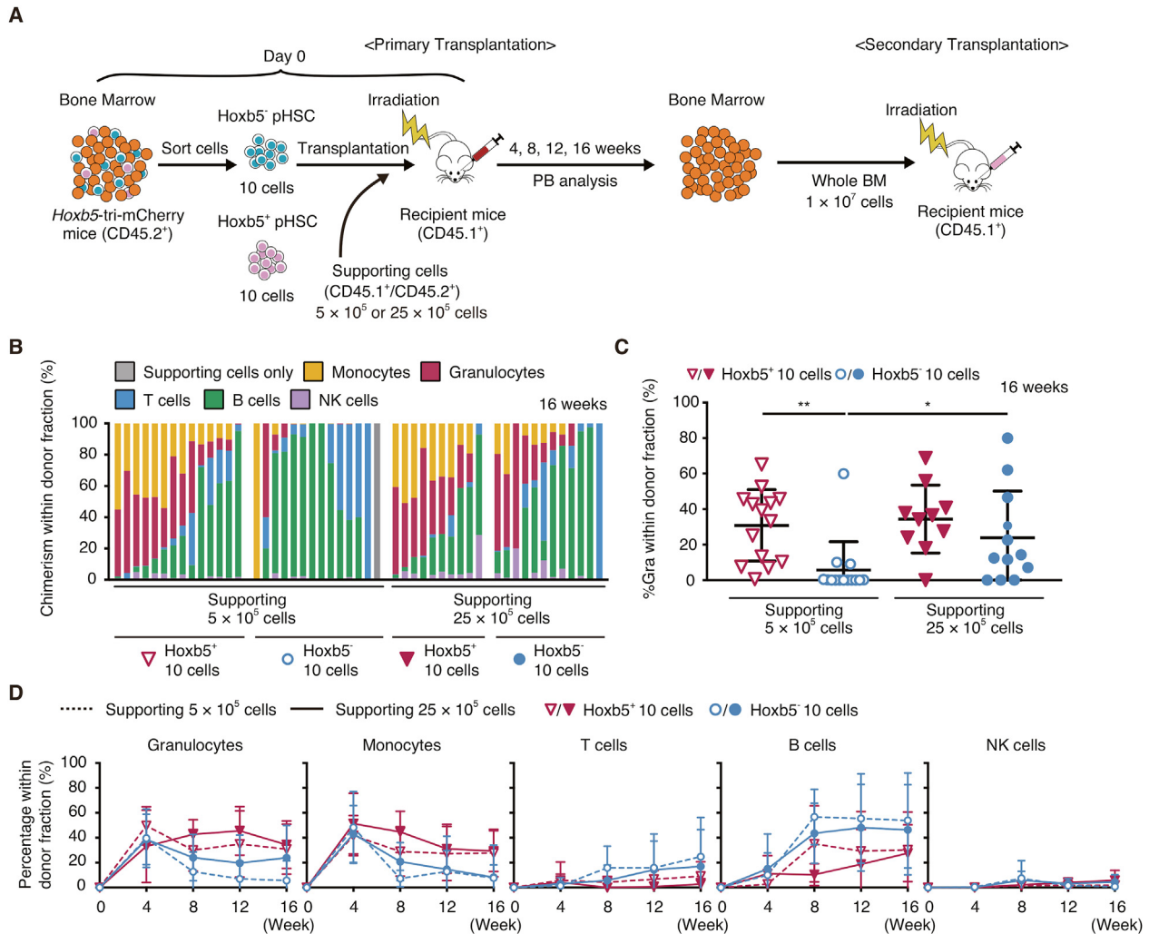
Fig. 3. Replication stress alters cell fate of Hoxb5 + pHSCs. (A) Experimental schematic for the stress titration assay. Ten donor cells (Hoxb5 + or Hoxb5 + pHSCs) were transplanted along with variable numbers of whole bone marrow (5 × 10 5 or 25 × 10 5 cells) from CD45.1/CD45.2 mice into lethally irradiated CD45.1 recipient mice. Peripheral blood was analyzed every four weeks. For secondary transplants, 1 × 10 7 whole bone marrow cells were transferred from the primary recipient mice. Peripheral blood was analyzed at 4, 12, and 33 weeks after secondary transplantation. (B) Reconstitution kinetics at 16 weeks in primary recipient mice. Each bar represents an individual mouse. (n = 14 for 10 Hoxb5 + pHSCs with 5 × 10 5 supporting cells; n = 14 for 10 Hoxb5 + pHSCs with 5 × 10 5 supporting cells; n = 10 for 10 Hoxb5 + pHSCs with 25 × 10 5 supporting cells; and n = 12 for 10 Hoxb5 + pHSCs with 25 × 10 5 supporting cells). (C) Granulocyte production at 16 weeks discussed in (B). (D) Average donor lineage kinetics in each group discussed in (A).
