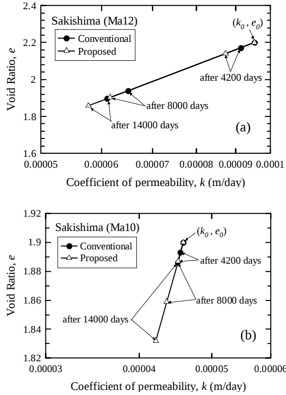
Fig. 9 Variation in coefficient of permeability with the decrease in void ratio
