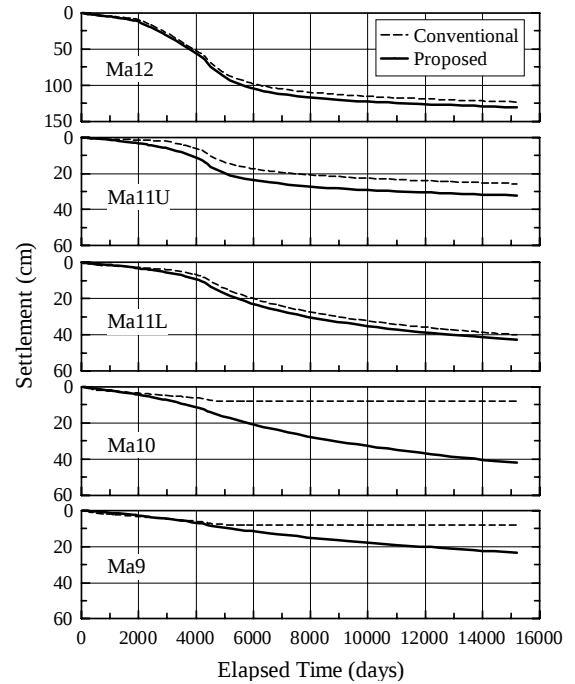
Fig. 13 Comparison of the calculated settlement for each Pleistocene clay layer of Yumeshima
