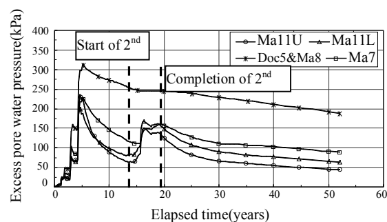
Fig. 9(d) Calculated performance of excess pore water pressure with time for the Pleistocene clay layers
