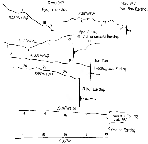
Fig. 1 (a). The Crustal Extensions at Osakayama before and after the Earthquakes of Ryujin, Ise-Bay, Hidakogawa, Fukui and Yoshino.
