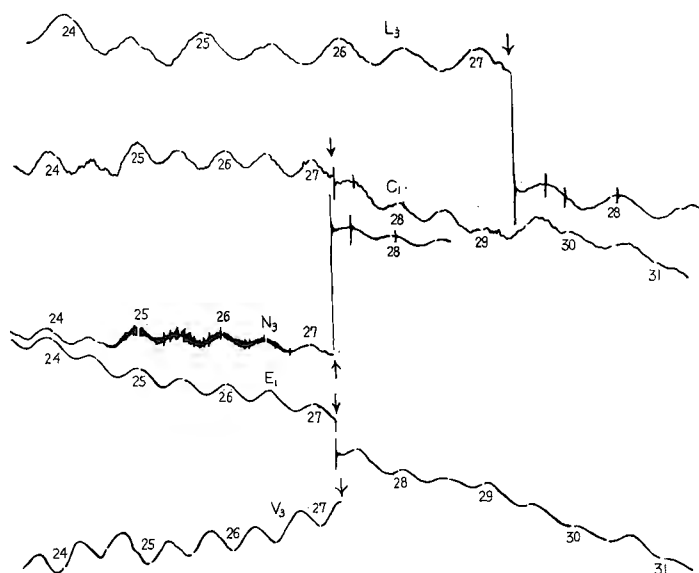
Fig. 1 (d). The Crustal Extensions at Osakayama before and after the off Echizen-misaki Earthquake.
