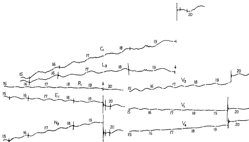
Fig. 1 (c). The Crustal Extensions at Osakayama before and after the Kitamino Earthquake.
