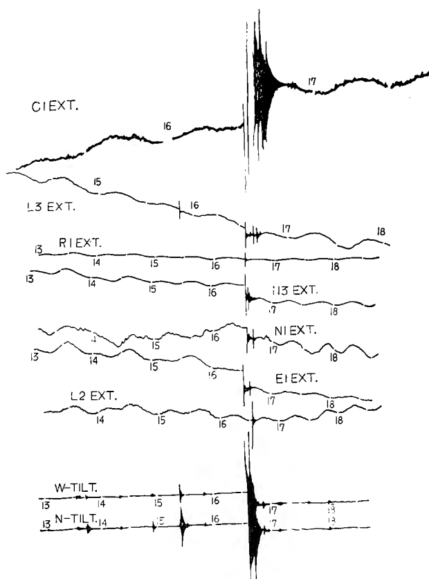
Fig. 1 (e). The Crustal Extensions and Tiltings at Osakayama before and after the Niigata Earthquake.
