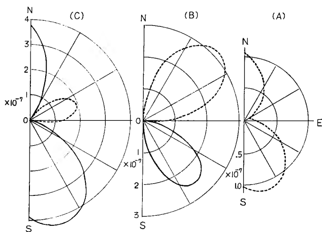
Fig. 3. The Azimuthal Pattern of the Abrupt Extensions at Osakayama in the Times of the Earthquakes of (A) Odaigahara, (B) Kitamino and (C) off Echizen-misaki. Solid Line is Extension and Dotted Line is Contraction.
