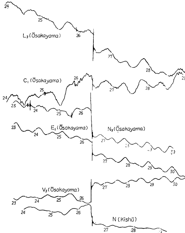
Fig. 1 (b). The Crustal Extensions at Osakayama and Kishu before and after the Odai-gahara Earthquake.
