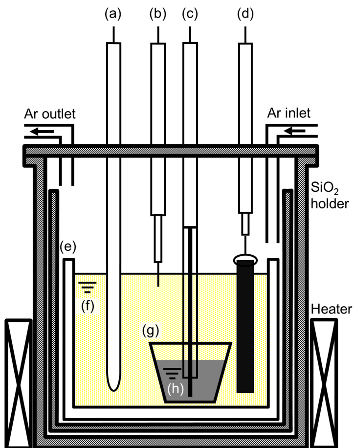
Figure 2. Schematic illustration of the electrolysis cell for observation of \text{SiO}_2 reduction behavior at liquid Zn cathode. (a) \text{Ag}^+/\text{Ag} reference electrode, (b) \text{Ca}^{2+}/\text{Ca} dynamic reference electrode on a Mo wire, (c) liquid Zn electrode with \text{Al}_2\text{O}_3/\text{SiO}_2 tube, (d) graphite counter electrode, (e) \text{Al}_2\text{O}_3 crucible, (f) molten \text{CaCl}_2 , (g) small \text{Al}_2\text{O}_3 crucible, and (h) liquid Zn.
