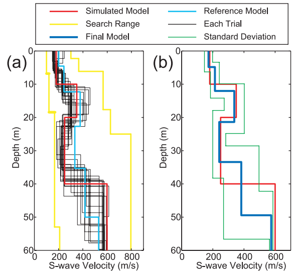
Figure 9. Results of inversions using effective phase velocities. (a) Simulated model (red), reference model constructed by eqs (14) and (15) (cyan), inverted models for each trial (black) and the search range in for the GA inversion (yellow). (b) Final inverted model (blue) obtained by averaging the S -wave velocities and thicknesses for each layer over 20 trials and their standard deviations (green).
