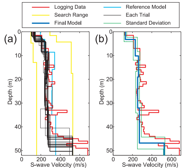
Figure 16. Results of inversions using SPAC coefficients. (a) Logging data (red), reference model constructed by eqs (14) and (15) (cyan), inverted models for each trial (black) and the search range for the GA inversion (yellow). (b) Final inverted model (blue) obtained by averaging the S -wave velocities and thicknesses for each layer over 20 trials and their standard deviations (green).
