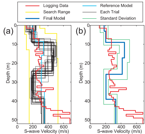
Figure 15. Results of inversions using effective phase velocities. (a) Logging data (red), reference model constructed by eqs (14) and (15) (cyan), inverted model for each trial (black) and the search range for the GA inversion (yellow). (b) Final inverted model obtained by averaging the S -wave velocities and thicknesses for each layer over 20 trials (blue) and their standard deviations (green).
