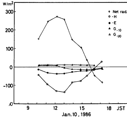
Fig. 3 An example of the variation of the heat fluxes. The fluxes are plotted as positive when they are toward the surface, and negative when off the surface.
