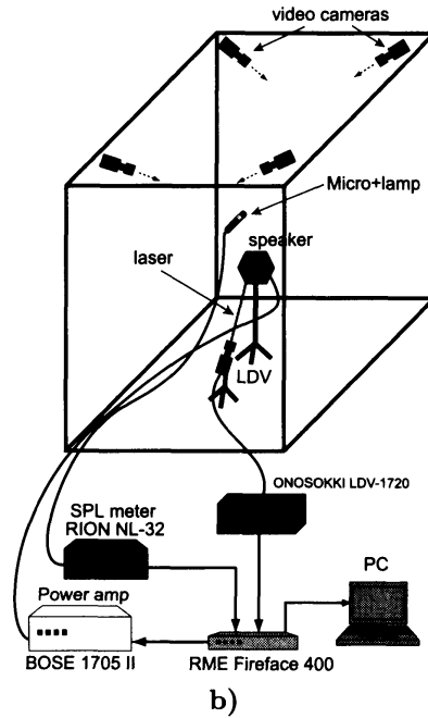
Figure 3: Measurement system.
