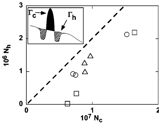
FIG. 7. The circulation \Gamma_h of ring holes is plotted as a function of the circulation \Gamma_c of the associated clump. The integrands \delta\zeta_b(x,y) and \bar{\zeta}_b(x,y) are schematically illustrated in the inset as hatched and dark regions, respectively. The symbols represent different sets of clumps in Fig. 6, \triangle for (a), \circ for (b), and \square for (c).
