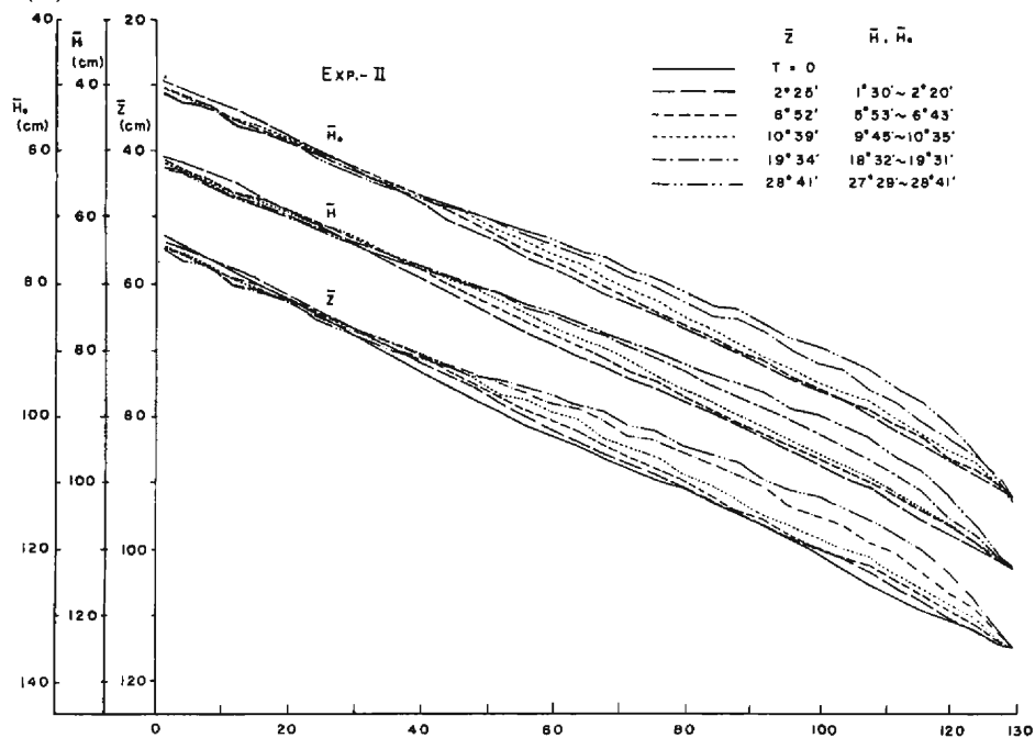
Fig. 3 Variation of water surface width of stream (c), and that of bed profile, water surface profile and energy head line (d) with time (Exp. II).
