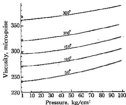
Fig. 7 Viscosity versus pressure diagram of argon
