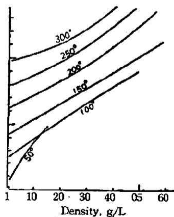
Fig. 4 Viscosity versus density diagram of ammonia
