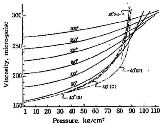
Fig. 1 Viscosity versus pressure diagram of \text{CO}_2
