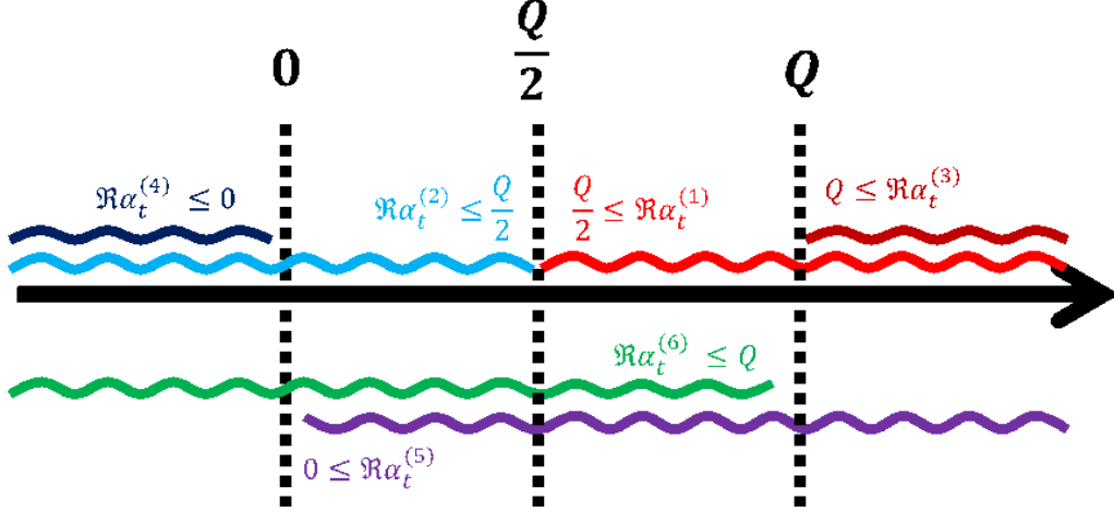
Figure 11. The domain of \Re\alpha_t^{(i)} . From this figure, we can find that only \alpha_t^{(5)} and \alpha_t^{(6)} can cross the contour \mathbb{S} of the integral over \alpha_t .
