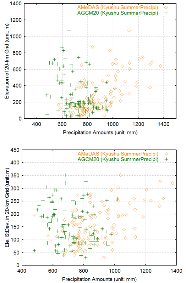
Fig. 7 Summer precipitation of Kyushu area, corresponding to the topographic information of the own grid; mean elevation (up) and standard deviation (down) of the elevation in the window.
