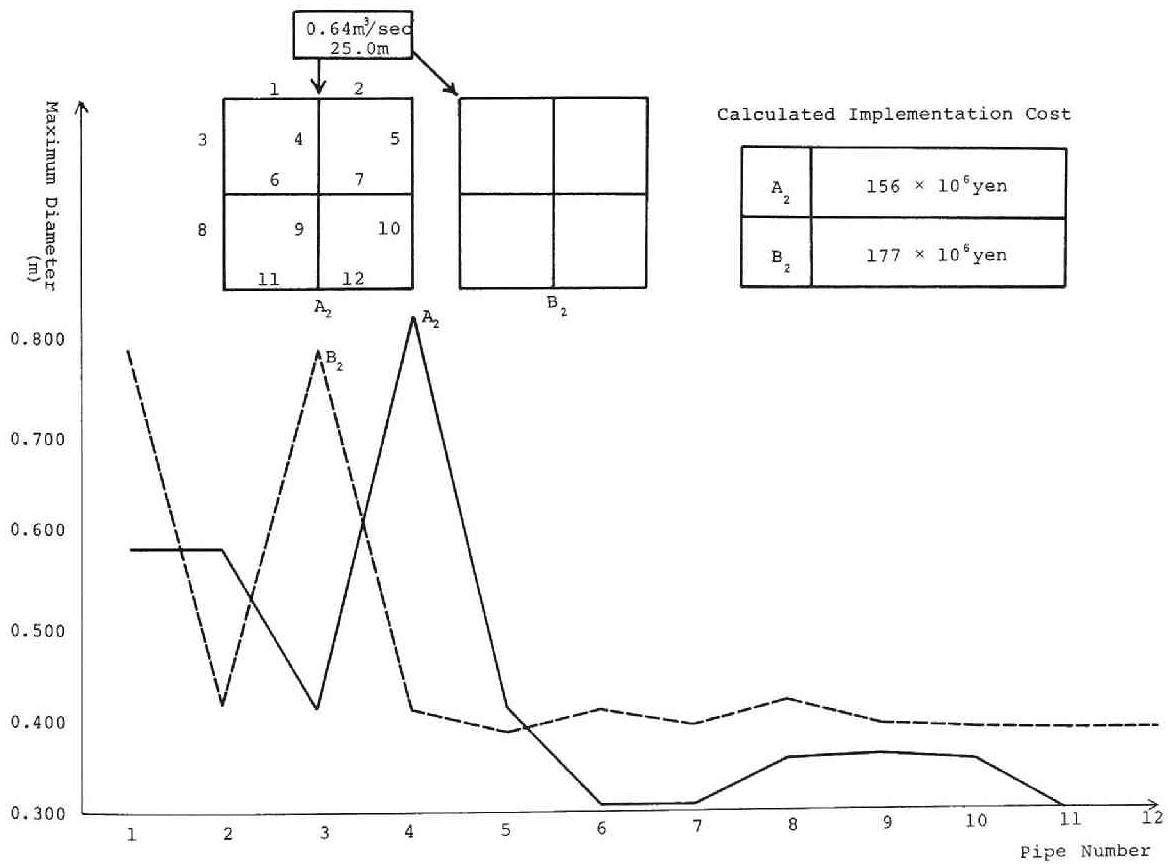
Fig. 6.9.4 Effect of Shift of Supply Node on Total Cost and Hydraulic Conditions
