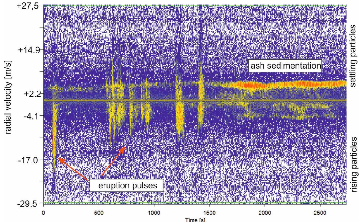
Figure 2: Spectrogram of an eruption on May 25th between 13:00 and 13:45:39 UTC shown as a function of time and radial velocity for activity above the Minamidake crater. Conversion of the radial velocities to vertical velocities is about 132.75 m/s and -123,75 m/s (minus is here upward, plus downward). Maximum vertical eruption velocities are about 80-85 m/s. Color codes the reflected energy given in dB.
