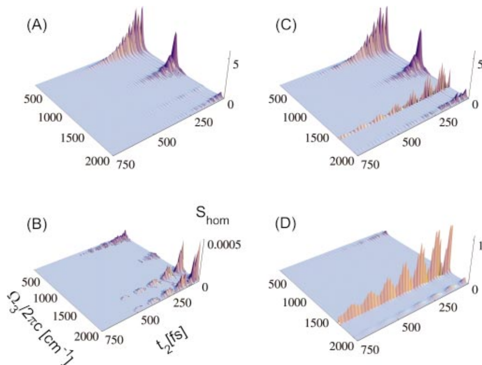
FIG. 6. (Color) Homodyne signal Eq. (20) for a system initially prepared in the nonequilibrium state (|2\rangle + |3\rangle)/\sqrt{2} . The BL [(a) and (b)] and the FR dynamics [(c) and (d)] is shown for t_1 = 0 [(a) and (c)] and t_1 = 1000 fs [(b) and (d)]. The relevant transitions frequencies are: \omega_{32} = 296 , \omega_{43} = 1048 , \omega_{21} = 1630 , and \omega_{30} = 1936 \text{cm}^{-1} . The system–bath parameters are: g_L = 0.19 , g_Q = 3 , \gamma_{pd} = 0 , and \omega_c/2\pi c = 500 \text{cm}^{-1} . Notice that the rather strong resonance at \Omega_3 = \omega_{10} is not shown for clarity.
