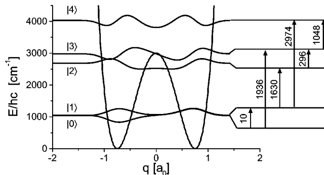
FIG. 1. Potential Eq. (1) with the lowest eigenstate wave functions at the respective eigenenergies for q_0 = 0.77a_0 and V_B/hc = 3000 \text{ cm}^{-1} . The dipole-allowed IR transitions according to Eq. (15) are shown as well (in \text{cm}^{-1} ). The coordinate matrix elements are \langle 0|q|1 \rangle = 0.71 , \langle 0|q|3 \rangle = 0.16 , \langle 1|q|2 \rangle = 0.18 , \langle 1|q|4 \rangle = 0.06 , \langle 2|q|3 \rangle = 0.5 , \langle 3|q|4 \rangle = 0.40 (in a_0 ). Equation (7) has been diagonalized using the Fourier Grid Hamiltonian method (Ref. 77) using 1024 grid points in the interval [-4a_0, 4a_0] . In the numerical solution of Eq. (6) the eight lowest states have been taken into account ( \omega_{70}/2\pi c = 6406 \text{ cm}^{-1} ).
