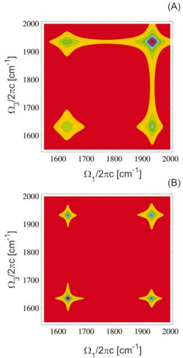
FIG. 5. (Color) Same as Figs. 3(a) and 3(c) but with inclusion of pure dephasing; BL—panel (a), FR—panel (b). The system—bath parameters are: g_L = 0.19 , g_Q = 1.1 , \gamma_{pd} = 0.005 , and \omega_c/2\pi c = 500 cm -1 .
