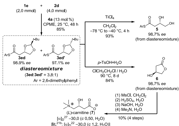
Scheme 2 Application of proposed protocol to asymmetric syntheses of \beta -hydroxy carboxyl compounds.
