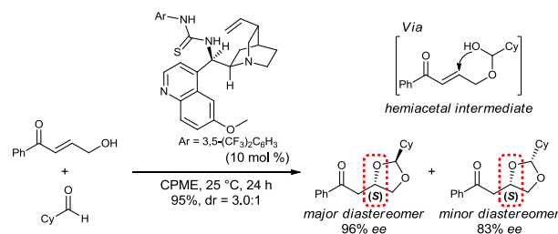
Scheme 1 Oxy-Michael addition via hemiacetal intermediates to \gamma -hydroxy- \alpha,\beta -unsaturated ketone via hemiacetal intermediate.
