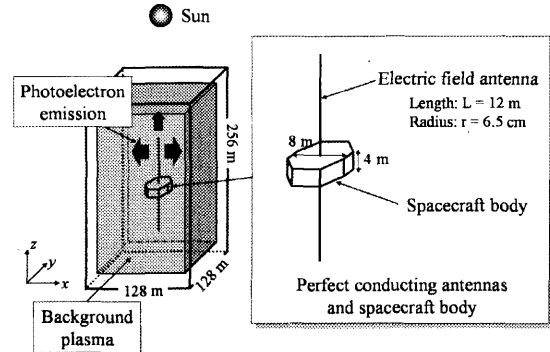
Figure 1: Simulation model.
