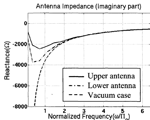
Figure 3: Imaginary part of impedance (reactance).
