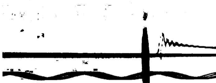
Fig. 4. No. 169. \text{H}_2:\text{O}_2=2:1 , P=3.50\text{ mmHg} (容器 No. 8, 薄膜 II.)
