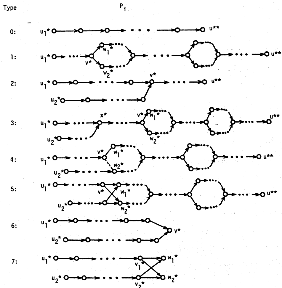
Fig. 6. Types of fundamental paths P_i determined in Step 3°-1.
