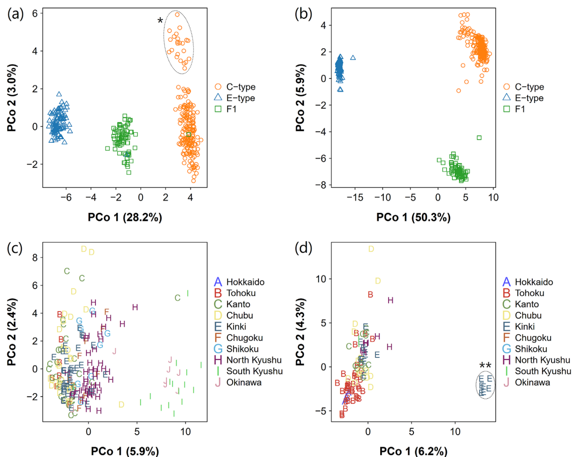
FIGURE 1 Principal coordinate analyses (PCoA) show genetic differentiation of Imperata cylindrica . (a) All accessions, except for accessions with a percentage of null loci over 30%. The minimum percentage of individuals across populations required to process a locus ( R ) was set to 0.8. The asterisk represents the Nansei population. (b) All accessions, except for accessions with a percentage of null loci over 70%. R was set to 0.5. (c) The C-type, except for the C-type with a percentage of null loci over 30%. R was set to 0.8. (d) The E-type, except for the E-type with a percentage of null loci over 30%. R was set to 0.8. Double asterisks represent the Yodogawa River accessions.
