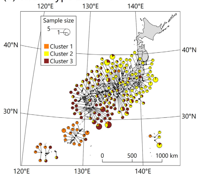
(b) The C-type at K = 3
