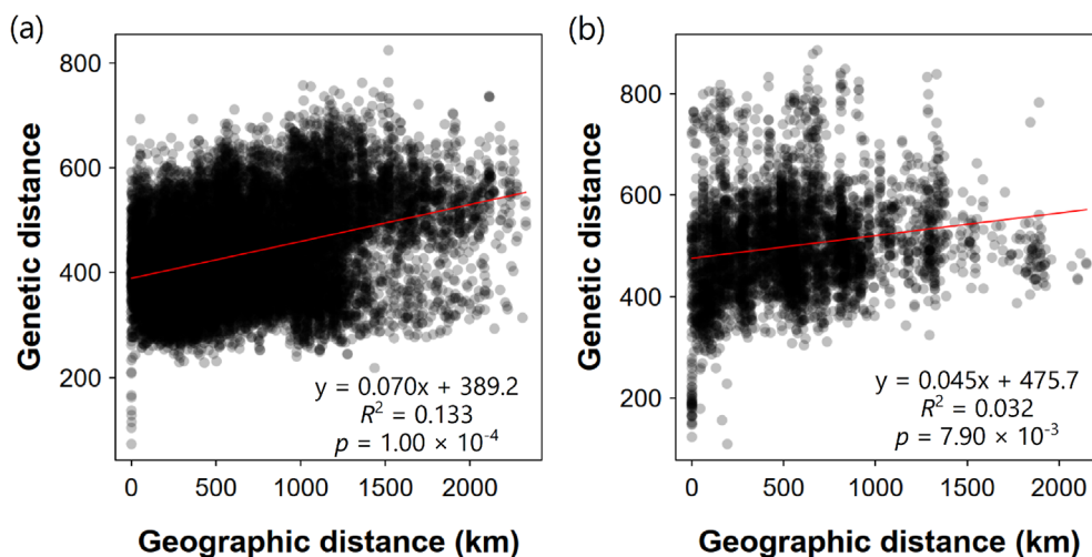
FIGURE 4 Mantel tests show the isolation by distance of two ecotypes of Imperata cylindrica . Mantel tests were conducted between genetic distance calculated using the GenAlEx algorithm and geographic distances for the (a) C-type and (b) E-type.
