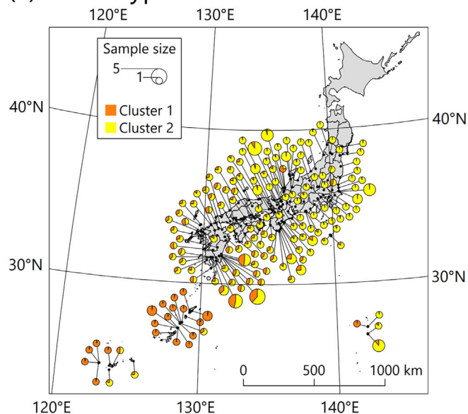
(a) The C-type at K = 2
