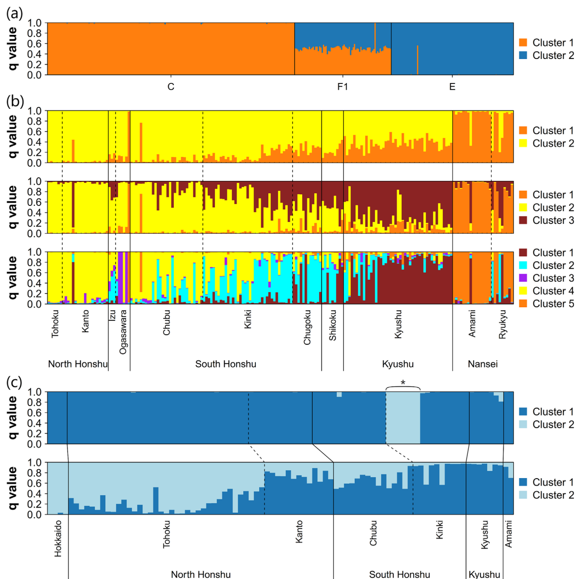
FIGURE 2 STRUCTURE analyses show genetic differentiation of Imperata cylindrica . (a) All accessions, except for those with a percentage of null loci over 30%. The minimum percentage of individuals across populations required to process a locus ( R ) was set to 0.8. (b) The C-type, except for those with a percentage of null loci over 30%. R was set to 0.8. The top, middle, and bottom are at K = 2 , K = 3 , and K = 5 , respectively. (c) The E-type, except for those with a percentage of null loci over 30%. R was set to 0.8. The top includes the Yodogawa River accessions. An asterisk represents the Yodogawa River accessions. The bottom excludes the Yodogawa River accessions.
