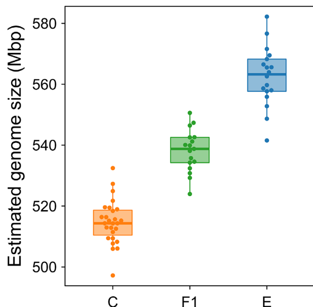
FIGURE 6 Genome sizes of the two ecotypes and F1 hybrid. Genome size was calculated as a relative value to the rice genome size (389 Mbp). The results of multiple comparisons are shown in Table S4. [Correction added on 19 December 2024, after first online publication: Figure 6 has been replaced in this version.]
