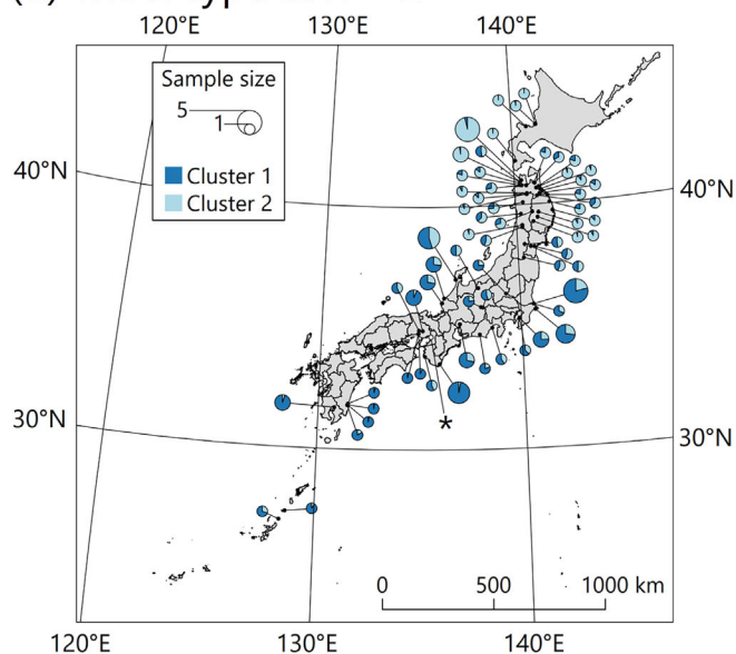
FIGURE 3 Distribution of each cluster in the STRUCTURE. (a–c) The C-type. The percentages of clusters in (a), (b), and (c) correspond to the STRUCTURE results in the top, middle, and bottom in Figure 2b, respectively. (d) The E-type. The percentage of clusters corresponds to the STRUCTURE results in Figure 2c. An asterisk represents the Yodogawa River population. The pie chart size represents the sample size.
