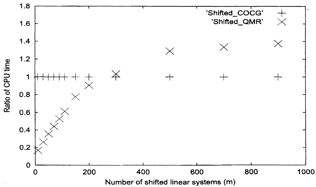
Figure 4: The ratio of the CPU time of the shifted QMR_SYM method to that of the shifted COCG method versus the number of shifted linear systems.
