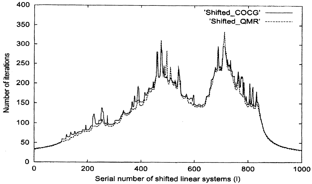
Figure 1: Number of iterations for the shifted COCG method and the shifted QMR_SYM method versus serial number of shifted linear systems.
