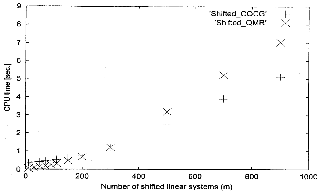
Figure 3: Required CPU time given in seconds versus the number of shifted linear systems for each iterative method.
