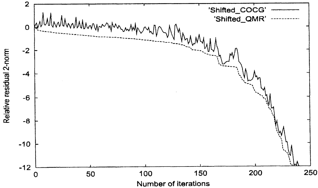
Figure 2: \text{Log}_{10} of relative residual 2-norms versus the number of iterations of the shifted COCG method and the shifted QMR_SYM method for shifted linear systems with \ell = 701 , i.e., \sigma_{701} = 1.100 + 0.001i .
