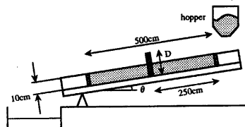
Fig. 1 Experimental flume
