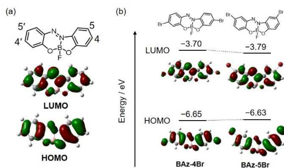
Figure 7. (a) Substituent positions of BAz-H . (b) Energy diagram and MOs of BAz-4Br and BAz-5Br with DFT calculation at B3LYP/6-311+G(2d,p) level (isovalue = 0.03). Reprinted with permission from ref 86. Copyright 2019 WILEY-VCH Verlag GmbH & Co. KGaA, Weinheim.
