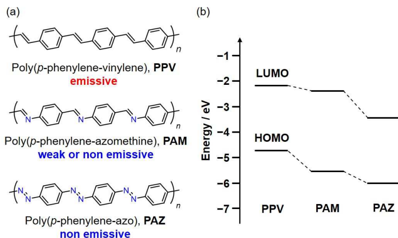
Figure 1. Structures and energy levels of HOMO and LUMO of \pi -conjugated polymers, PPV, PAM and PAZ. Reprinted with permission from ref 20. Copyright 2005 Elsevier.
