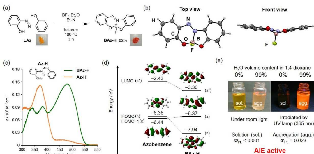
Figure 4. The functionalities of BAz-H . (a) Synthesis of BAz-H from LAz and their colors. (b) ORTEP drawings of BAz-H from results of single crystal X-ray structural analysis. (c) UV-vis absorption spectra of BAz-H and Az-H in toluene ( 1.0 \times 10^{-5} M). (d) Energy diagram, selected MOs of azobenzene and BAz-H with DFT calculation at B3LYP/6-311G(d,p) level (isovalue = 0.03). (e) AIE properties of BAz-H . Reprinted with permission from ref 46. Copyright 2018 WILEY-VCH Verlag GmbH & Co. KGaA, Weinheim.
