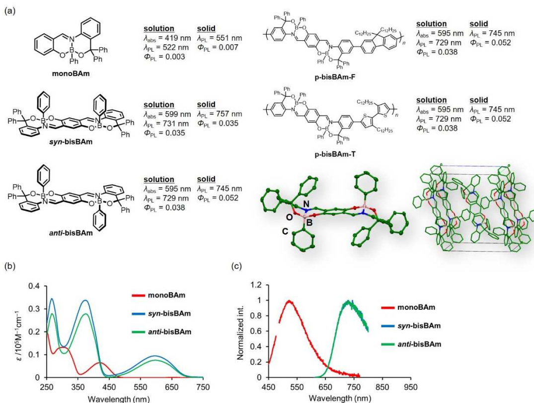
Figure 13. (a) Structures and optical properties of monoBAm , bisBAm and polymers, and an ORTEP drawing and a crystal packing of anti-bisBAm where hydrogen atoms are omitted for clarity. (b) UV–vis–NIR absorption and (c) emission spectra of monoBAm and bisBAm in chloroform ( 1.0 \times 10^{-5} \text{ M} ). Reprinted with permission from ref 103. Copyright 2020 The Royal Society of Chemistry.
