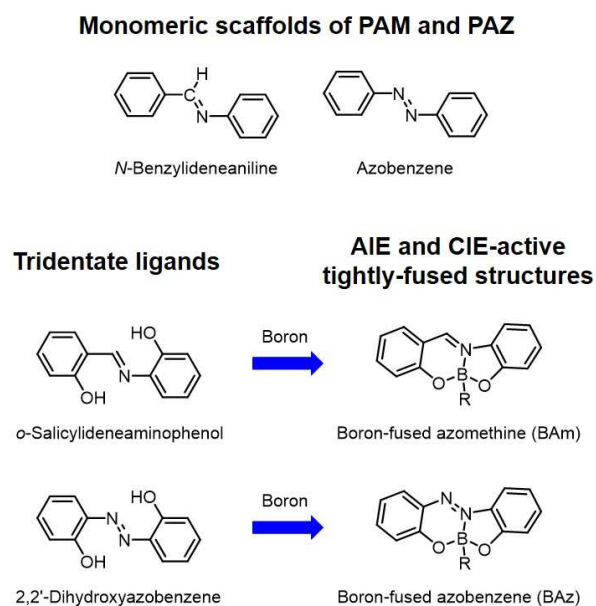
Figure 2. Structures of the azomethine and azobenzene derivatives and boron complexes with O,N,O-type tridentate ligands. Reprinted with permission from ref 50. Copyright 2019 The Chemical Society of Japan.
