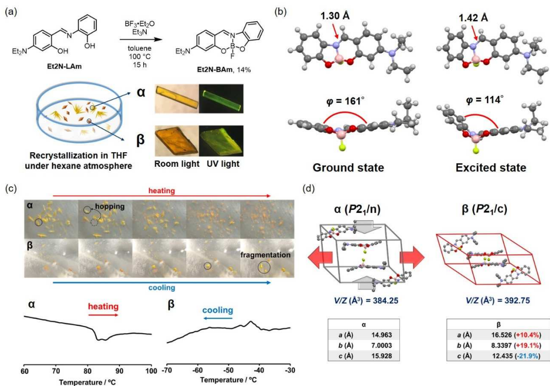
Figure 11. (a) Synthesis of Et2N-BAm and separation of the polymorph. (b) Optimized structures in the ground and excited states of Et2N-BAm with DFT and TD-DFT calculations at the B3LYP/6-311G(d,p) and TD-B3LYP/6-311+G(d,p) levels, respectively. (c) Snapshots of thermosalient behaviors and DSC curves of crystal \alpha and \beta . (d) Anisotropic deformation of unit cells of \alpha and \beta during \alpha \rightarrow \beta crystal-crystal transition. Reprinted with permission from ref 45. Copyright 2017 WILEY-VCH Verlag GmbH & Co. KGaA, Weinheim.
