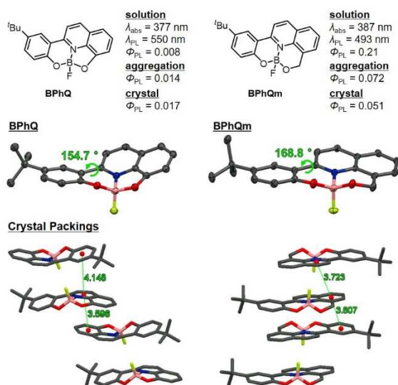
Figure 14. Structures, optical properties, ORTEP drawings and crystal packing structures of BPhQ and BPhQm . Hydrogen atoms are omitted for clarity. Reprinted with permission from ref 104. Copyright 2020 MDPI (Basel, Switzerland).
