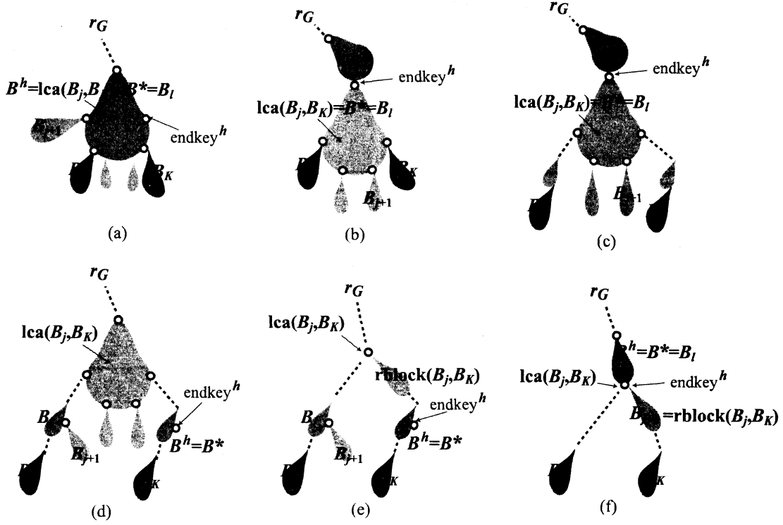
Figure 4: Illustration for the six subcases of the case where the tip-block B_K = B^p has the competitor B_j with \gamma'(B_j) \simeq \gamma'(B_K) .
