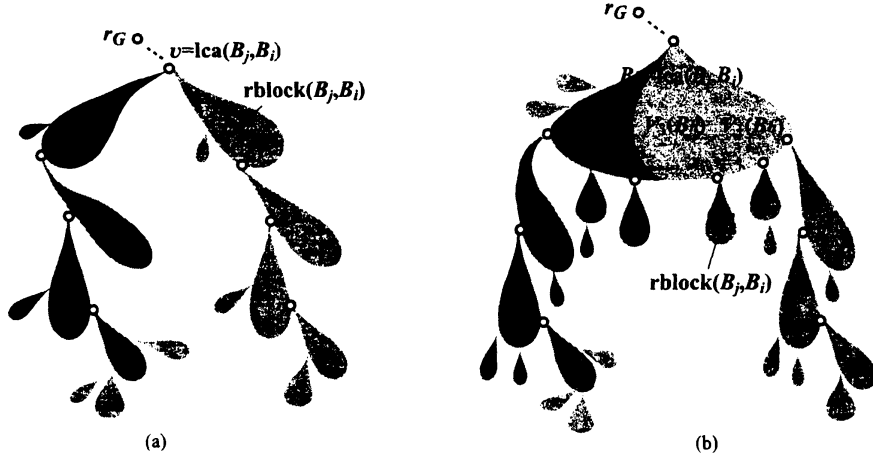
Figure 2: Two possible cases where a block B_j is pre-identical to a block B_i , (a) \text{lca}(B_i, B_j) is a vertex v ; (b) \text{lca}(B_i, B_j) is a block B_h .
