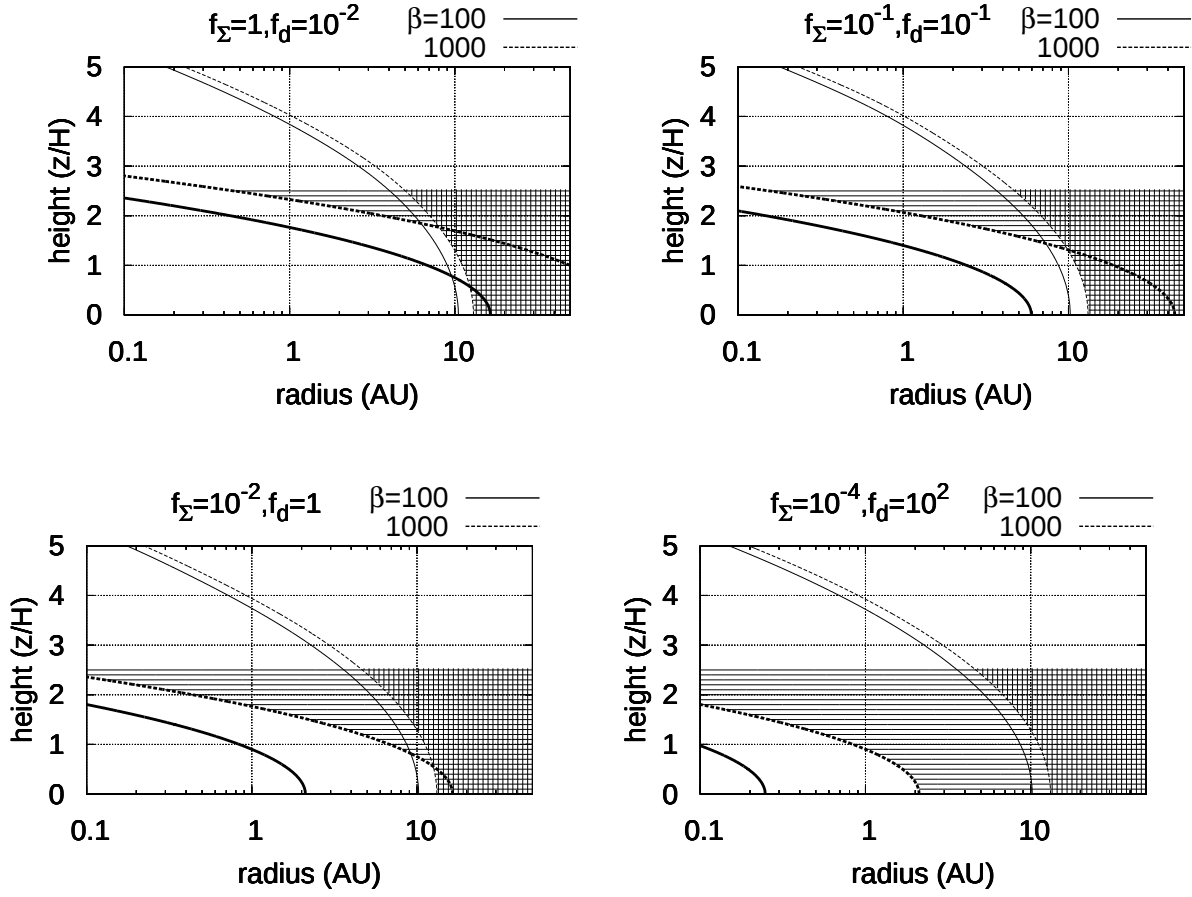
Fig. 9.— Change of unstable regions as the gas density of the disk decreases, while the dust density is kept constant. The MRI-unstable region according to (SMUN00) and our model, while marked by vertical and horizontal stripes, respectively, for \beta = 1000 .
