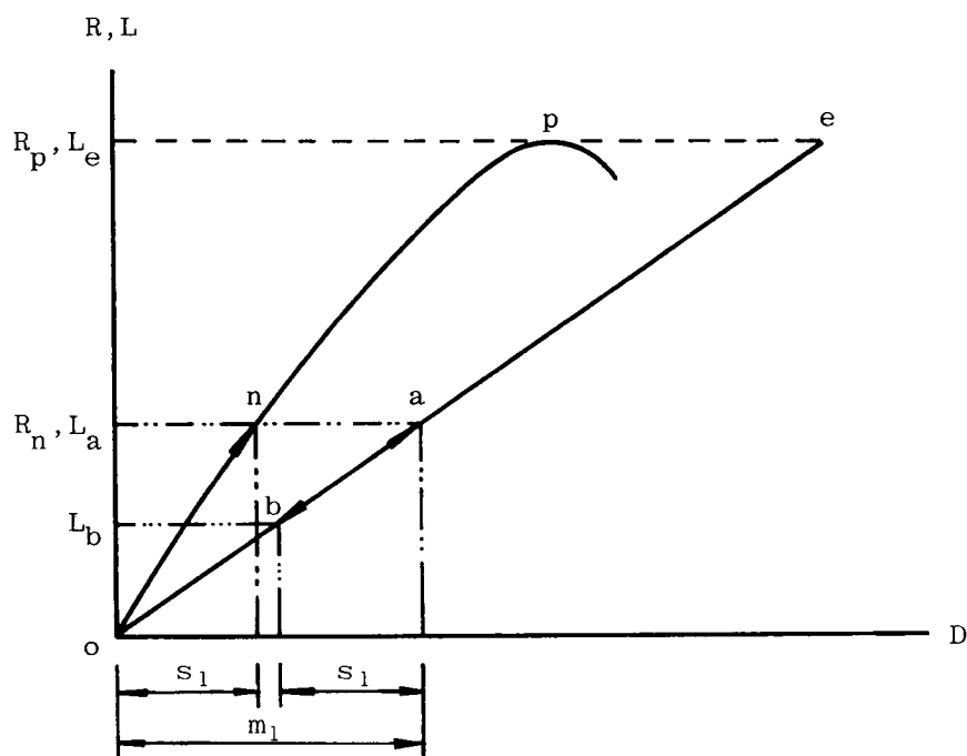
Fig.A-9 Shear test using a less stiff loading machine before peak strength point
