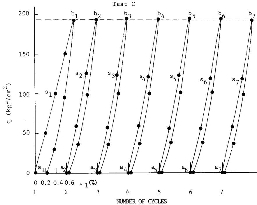
Fig. 6-3 The relationship between q - \epsilon_1 versus number of cycles of Test C (ultimate cyclic loading = 0.8 \times q_{\text{peak}} ).
