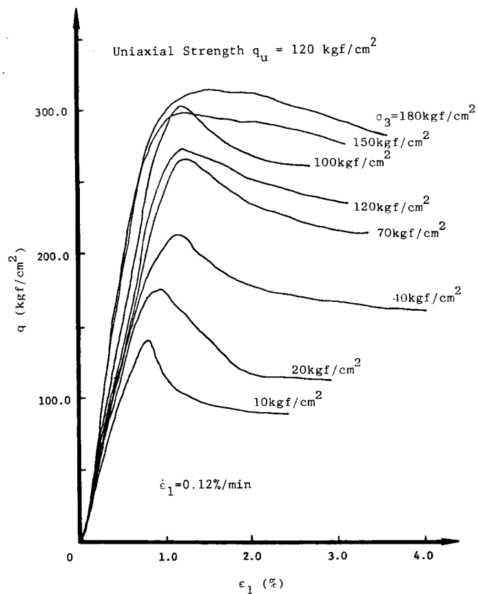
Fig. 3-2-5(a) q - \epsilon_1 relationships of Funyu rock (Ref. 3-12)
