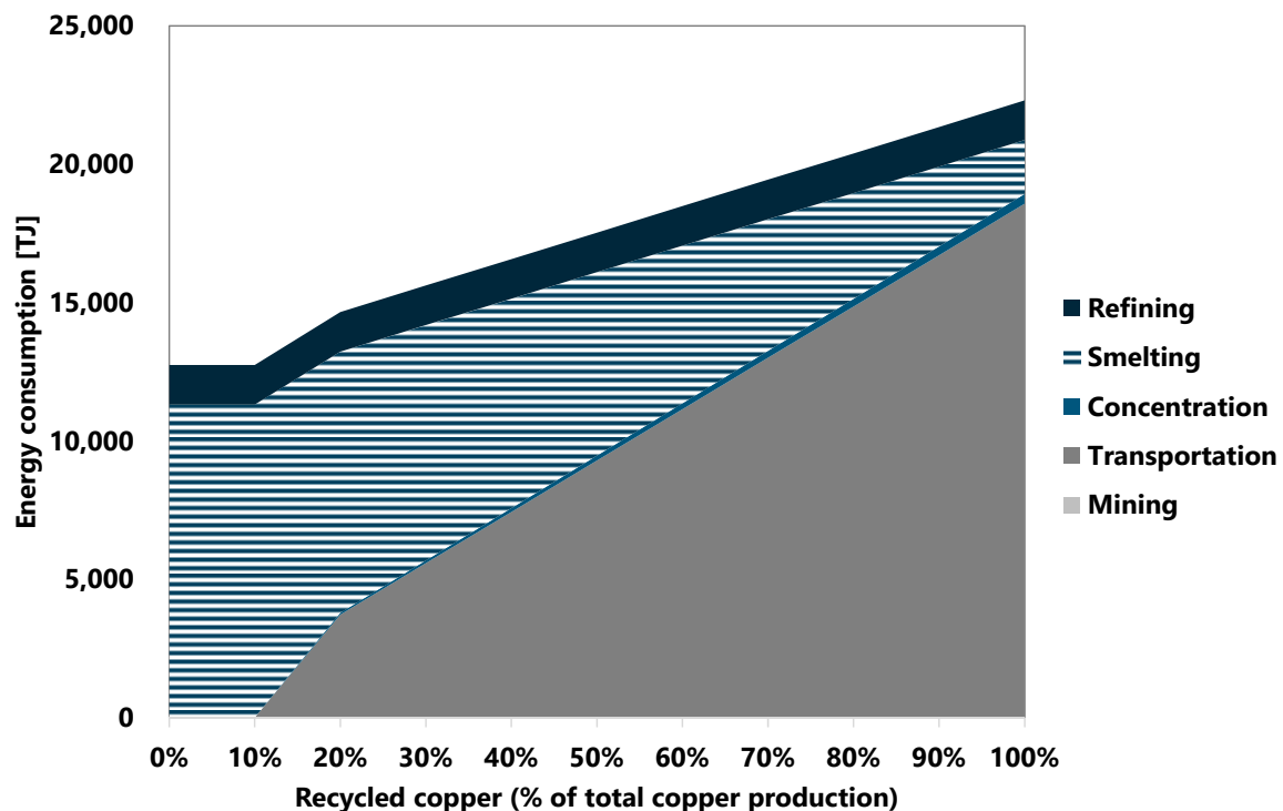
Figure 6. Final energy consumption in a recycling society.
