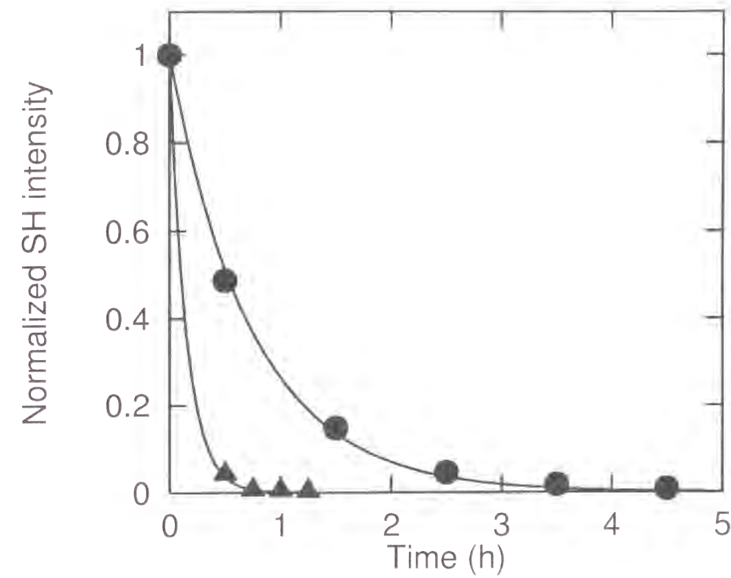
Fig. 3.4: Relaxation behavior of second-harmonic generation measured at elevated temperatures for 20\text{WO}_3\cdot 80\text{TeO}_2 glasses poled at 260 °C. The closed circles and triangles denote the normalized second-harmonic intensity measured at 100 and 150 °C, respectively. The experimental data were fitted using Eq. (2.1) with \tau and \beta listed in Table 3.2.
