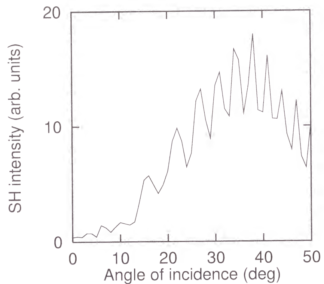
Fig. 1.3: Maker fringe pattern of 30\text{NaO}_{\frac{1}{2}}\cdot 70\text{TeO}_2 glass poled at 220^\circ\text{C} with 3 kV.
