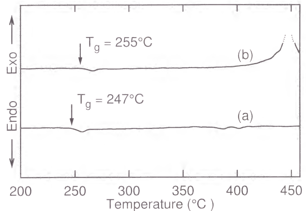
Fig. 1.11: Differential scanning calorimetry curves of (a) 10\text{Li}_2\text{O}\cdot 10\text{Na}_2\text{O}\cdot 80\text{TeO}_2 glass and (b) 18\text{Na}_2\text{O}\cdot 82\text{TeO}_2 glass.
