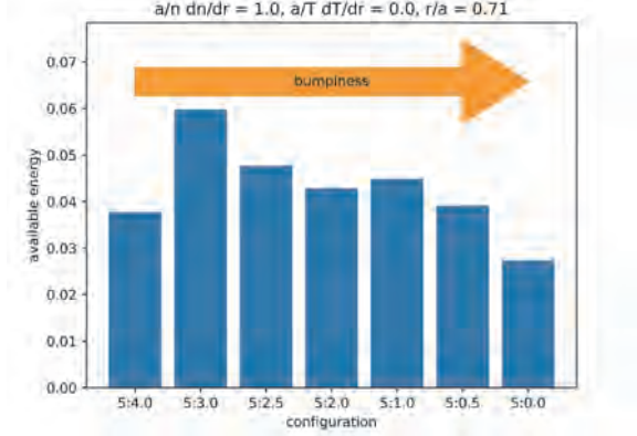
Figure 3: Available energy calculated for the different configurations of Heliotron J for a density gradient a/Ln=3 .
