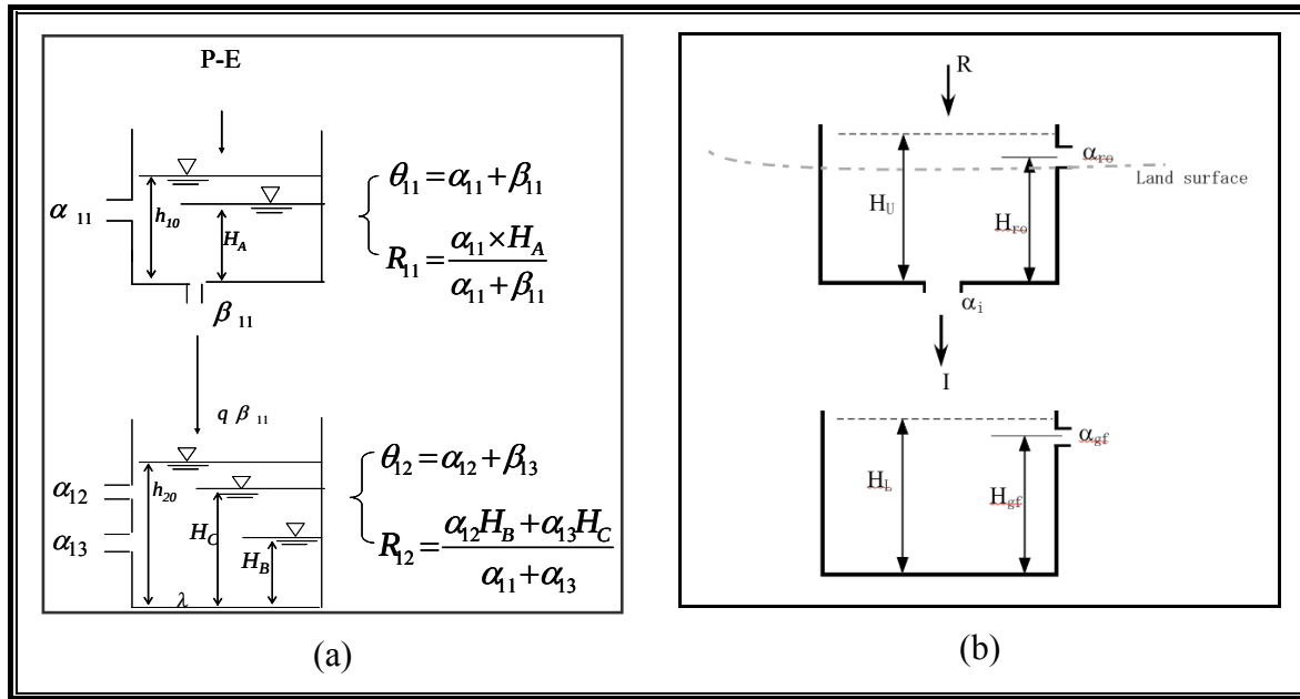
Figure 6.2 Configuration of tank model. (a) The original of tank model, and (b) the modification of tank model.
