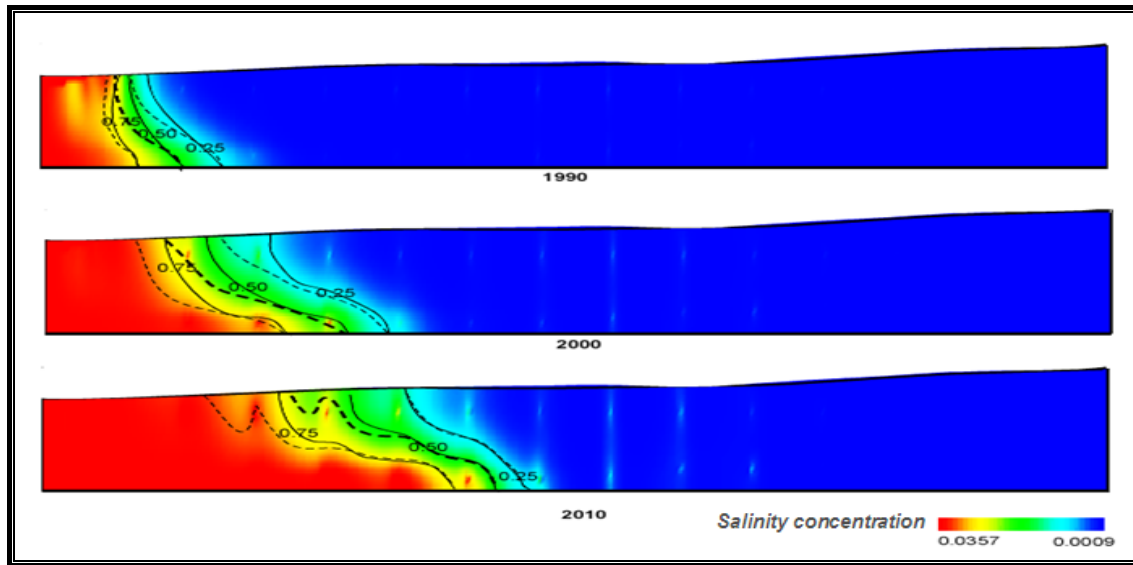
Figure 4.19 The simulated interface form with infiltration rate of 2 \times 10^{-6} kg/m/sec.
