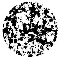
d) Schall: 39 \text{ W/cm}^2 L = 4 \text{ mm}
