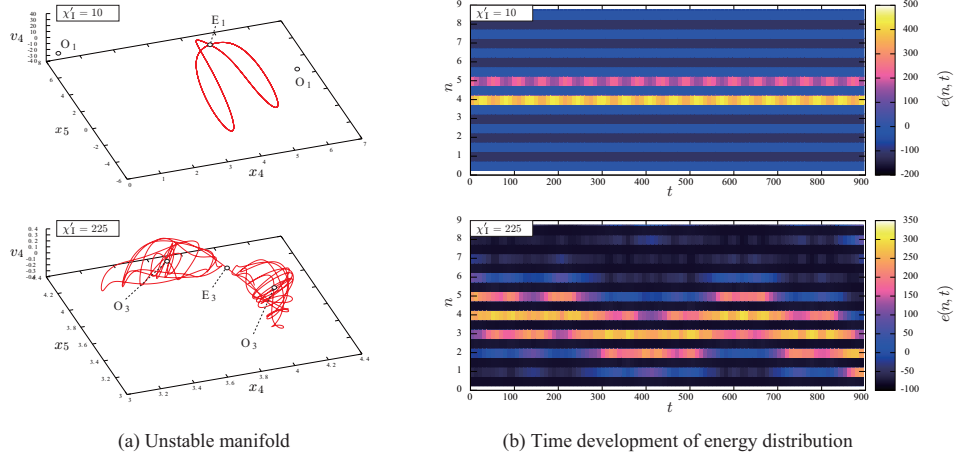
FIGURE 3. Unstable manifolds and time development of energy distribution of the perturbed ILMs
