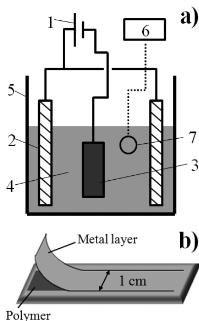
Figure 2.3. (a) A schematic diagram of the Cu electroplating apparatus: 1) DC power supply; 2) Anode; 3) Cathode (Ni-P plated polymer); 4) Plating solution; 5) Glass bath; 6) Air pump; 7) Air bubble stone; (b) Prepared sample for peeling-test machine
