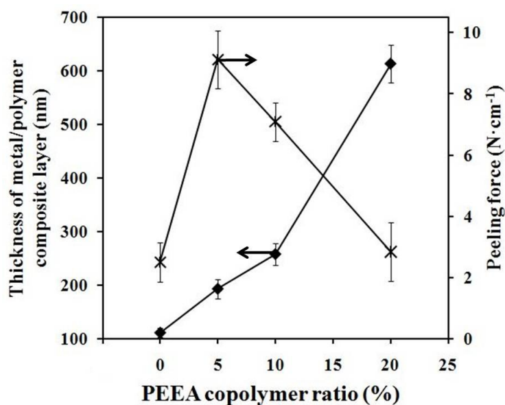
Figure 4.17. Relationship between weight percentage of PEEA copolymer in blend and thickness of metal-polymer composite layer and peeling force
