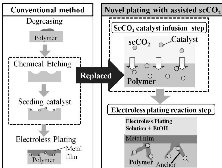
Figure 2.1. Schematics of conventional and developed scCO 2 -assisted electroless plating processes
