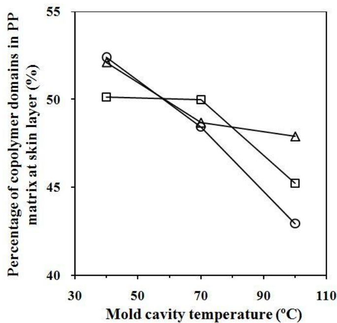
Figure 3.11. Effect of the mold cavity temperature on the average percentage of the PP-b-PEO copolymer domains in PP matrix (PP/PP-b-PEO (75/25) blend samples: \square = rPP; \circ = iPP-B; \Delta = iPP-A)
