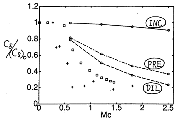
図 15. 混合層の拡大率 (+ Papamoshou &amp; Roshko, □ Langley experimental curve)
