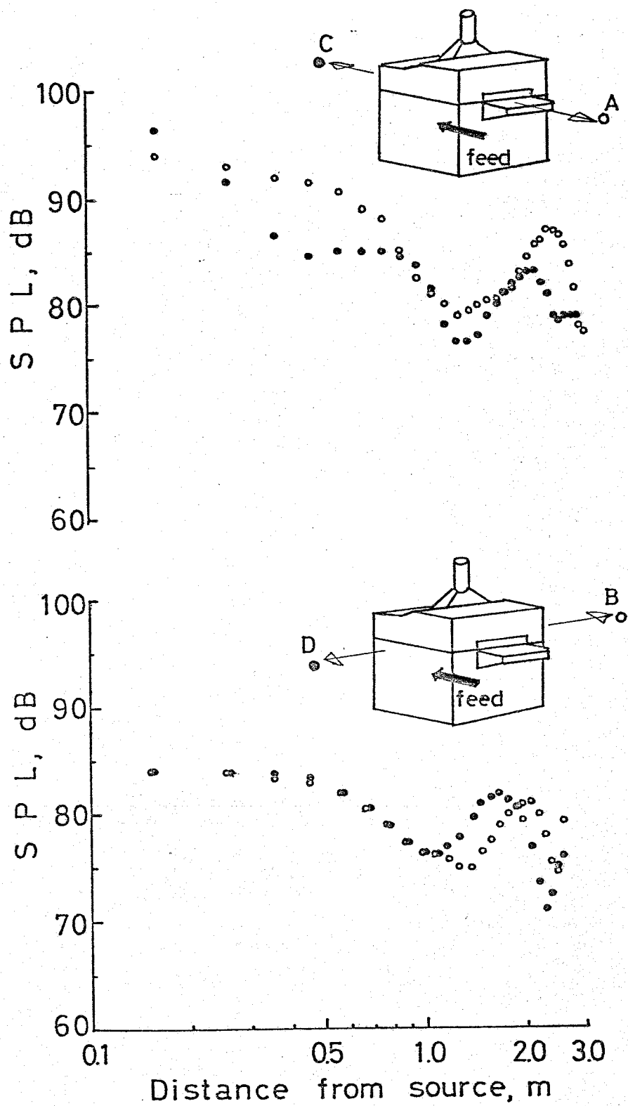
Fig. 2-1-6 SPL versus distance from source. The room was excited by single surface planar noise.
