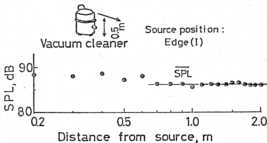
Fig. 3-3-5 SPL versus distance from source (vacuum cleaner) in the reverberant test room. The sound source was located at the edge (I).
