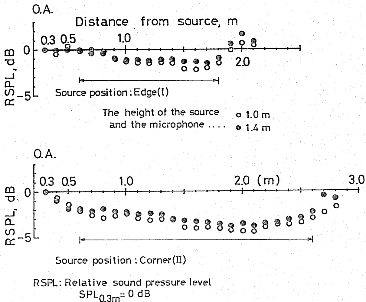
Fig. 2-4-4 SPL (O.A.level) versus distance from source. Broad band random noise was radiated from an isotropic sound source located at the edge (I) or the corner (II) at the height of 1.0 m or 1.4 m from the floor.
