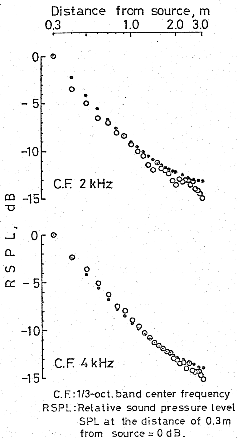
Fig. 2-1-12 One-third oct. band SPL versus distance from source. 2 kHz- and 4 kHz-band levels were measured.
