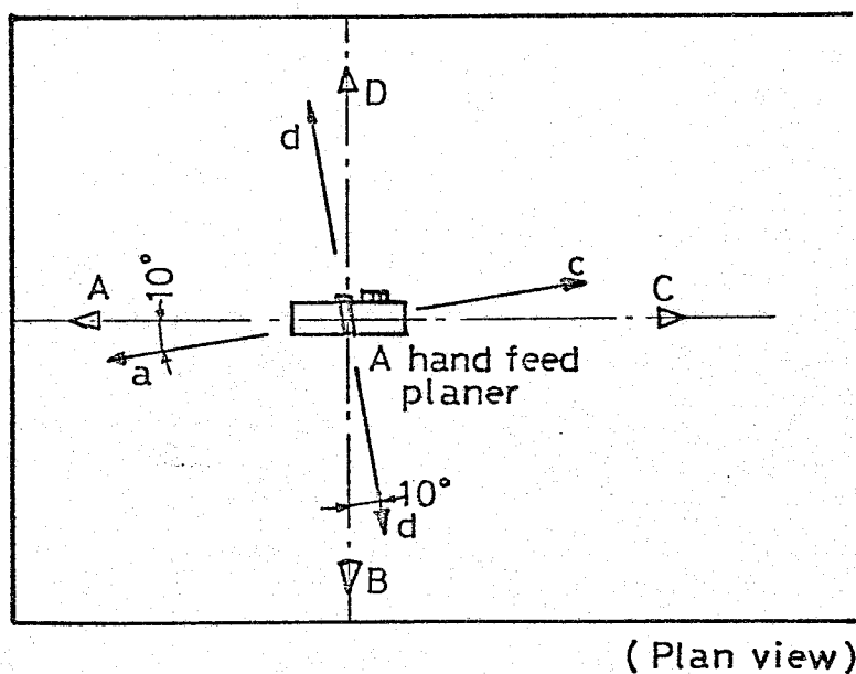
Fig. 2-1-4 The measuring directions in case of the hand feed planer source. The cutter-head of it was attached to the frame with a slant of 10 deg.
