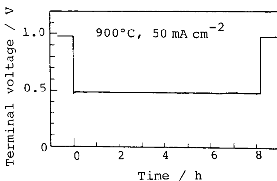
Fig. 27 Continuous discharge test of the fuel cell; \text{H}_2, \text{Ni} \mid \text{SrCe}_{0.95}\text{Yb}_{0.05}\text{O}_{3-\alpha} \mid \text{La}_{0.4}\text{Sr}_{0.6}\text{CoO}_{3-\alpha}, \text{O}_2
