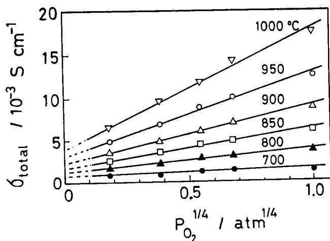
Fig. 60 Plots of total conductivity of SrCe_{0.95}Yb_{0.05}O_{3-\alpha} against P_{O_2}^{1/4} . P_{H_2O} = 6.03 \times 10^{-3} atm
