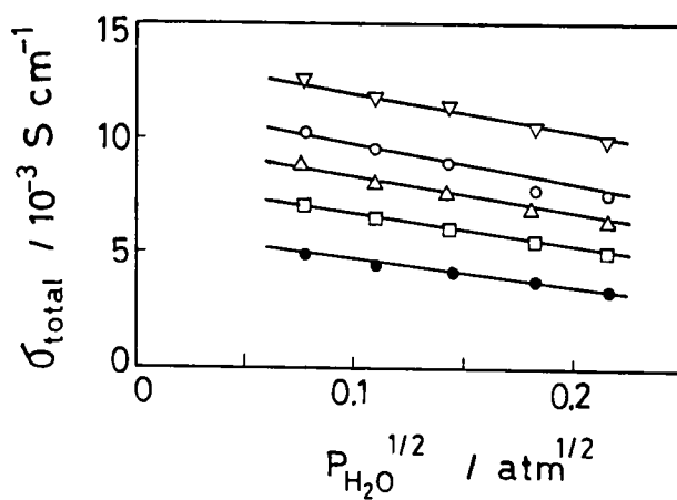
Fig. 59 Plots of total conductivity against P_{H_2O}^{1/2} at 950°C. P_{O_2} (\text{atm}) ; \nabla :1.0, \circ :0.21, \Delta :0.0673, \square :0.0218, \bullet : 1.07 \times 10^{-3}
