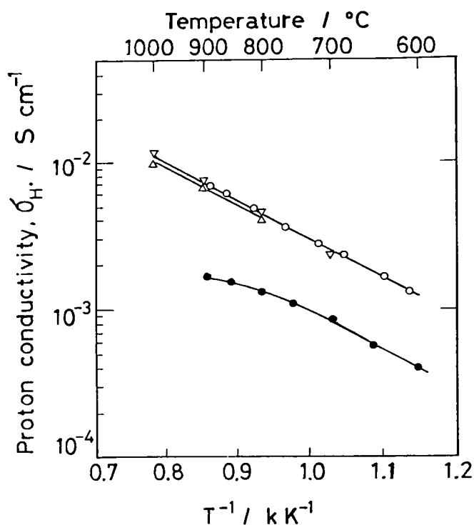
Fig. 64 Proton conductivity of \text{SrCe}_{0.95}\text{Yb}_{0.05}\text{O}_{3-\alpha}
