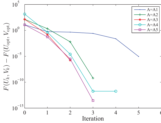
Figure 5.4.1: The differences between the optimal and the current values of the objective functions with A = A_1, A_2, \dots, A_5 .
