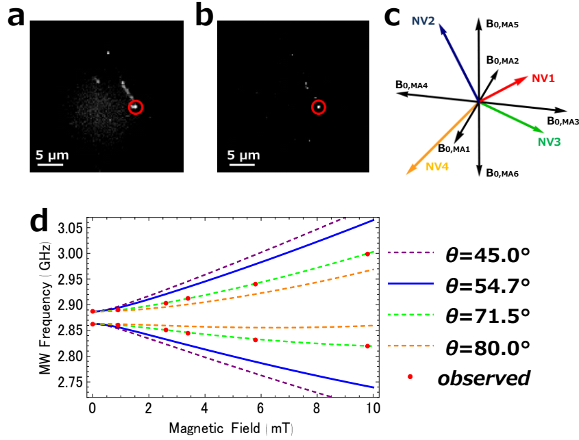
Figure 4-5 a,b, Fluorescence images of FNDs on a coverslip without (a) and with (b) selective imaging protocol. The fluorescent spot indicated by a red circle is an FND containing of single NVC. a,b are created by the same procedure for Figure 2b,c from 32 consecutive images (EMCCD exposure = 50 ms). c, Schematic drawing of the possible four orientations of a NVC in FND and our definition of angles ( \theta , \phi ) between a NVC orientation and the externally applied magnetic field H_0 . d, MW frequency of a pair of dips observed from an FND (red points) under 6 external magnetic field with different magnitudes (0, 0.9, 2.6, 3.4, 5.8, and 9.8 mT) and MW frequency simulated for several angle conditions.
