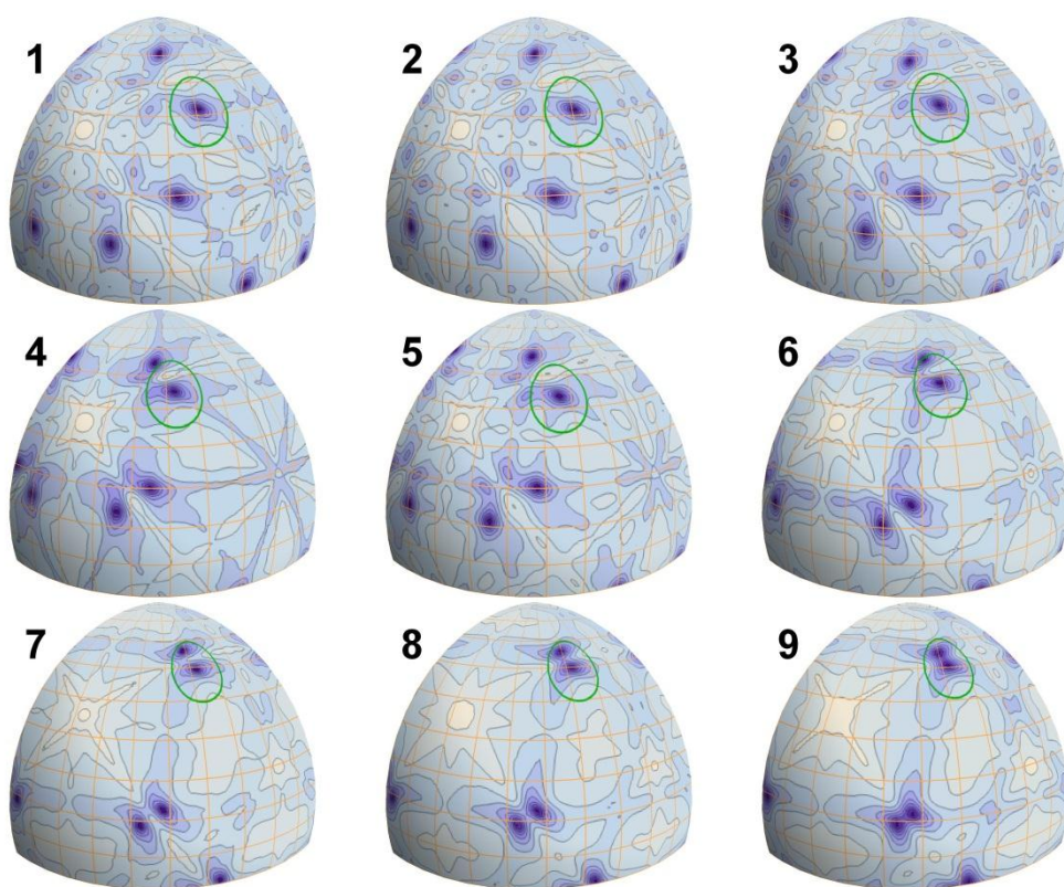
Figure 4-13c One-quarter hemispherical density maps of the residue in the non-linear least-square fit of the rotational angles ( \theta , \phi ) of an FND inside living itr-1 ( sa73 ) mutant.
