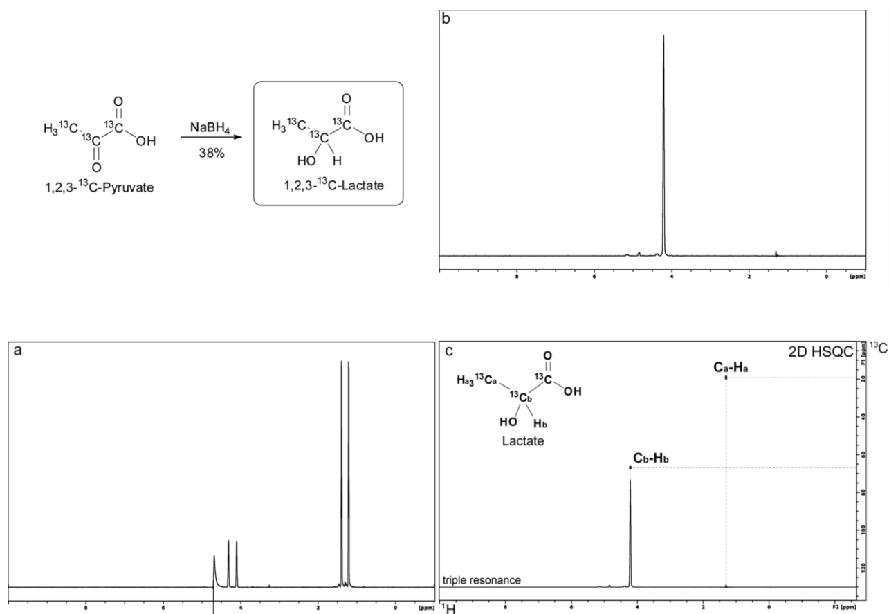
Figure 2-2 NMR spectra of chemically synthesized ^{13}\text{C}_3 -lactate. a) Single ^1\text{H} , b) triple resonance ^1\text{H}-\{^{13}\text{C}-^{13}\text{CO}\} and c) 2D ^1\text{H}-^{13}\text{C} HSQC spectra of chemically synthesized lactate (1 mM) in \text{D}_2\text{O} . The 2D HSQC spectrum c) is merged with the 1D ^1\text{H}-\{^{13}\text{C}-^{13}\text{CO}\} triple resonance spectrum b).
